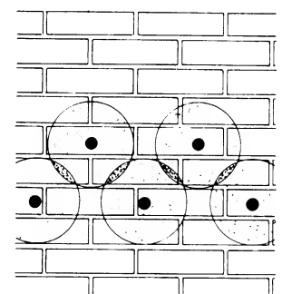
⑨ Injected damp-proofing
